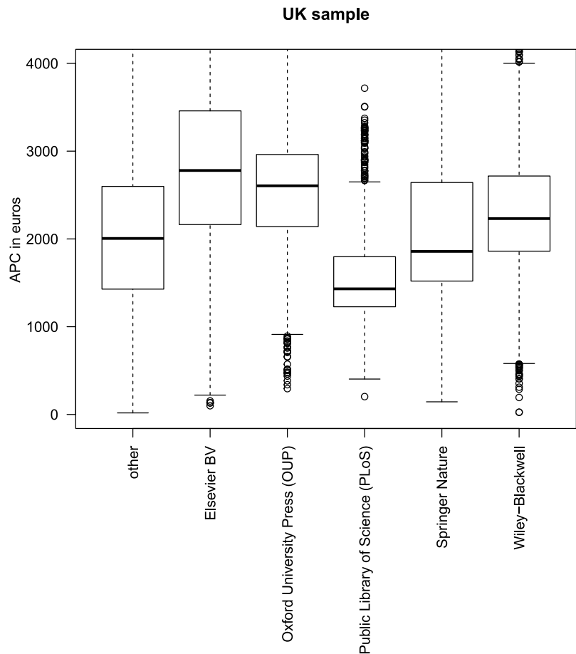
Figure 7. Box plots of APC for each publisher. Note: Some APCs are out of scale.
