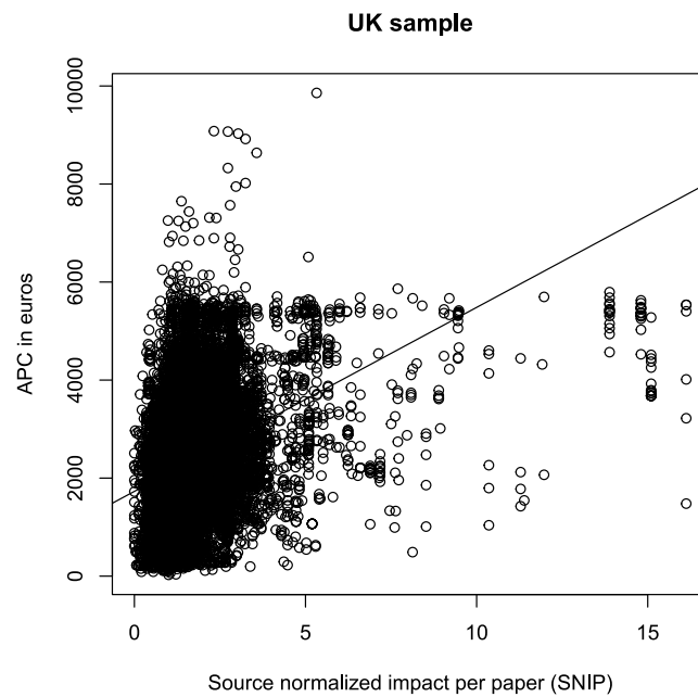
Figure 3. Scatter plot APC vs. SNIP.
