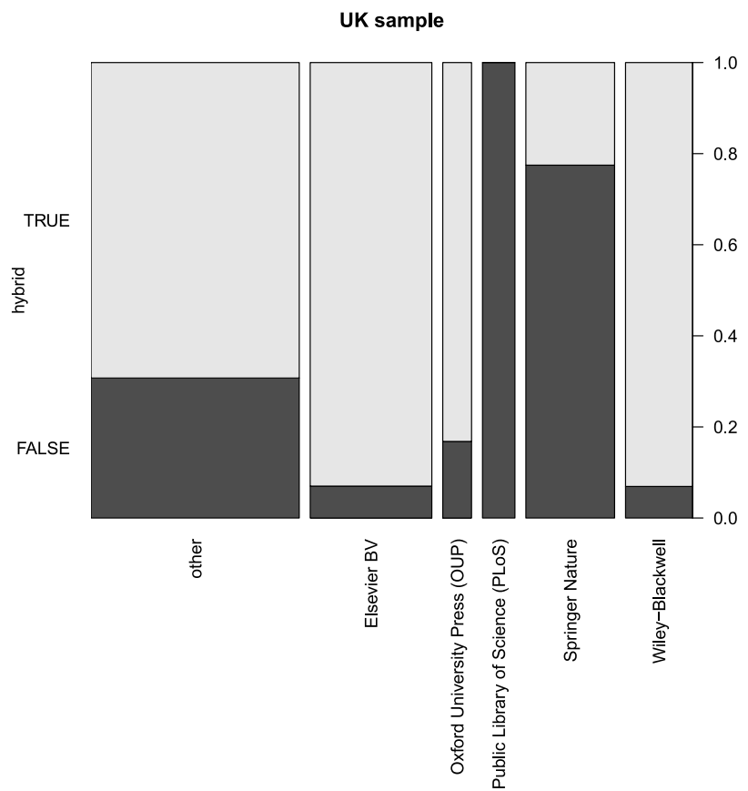
Figure 6. Distribution of articles among publishers and open-access vs. hybrid journals.
