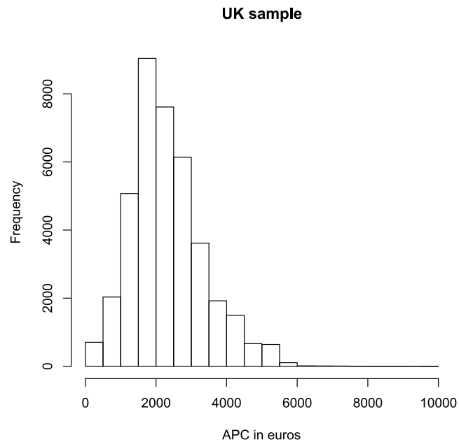
Figure 2. Histogram of APC in euros.
