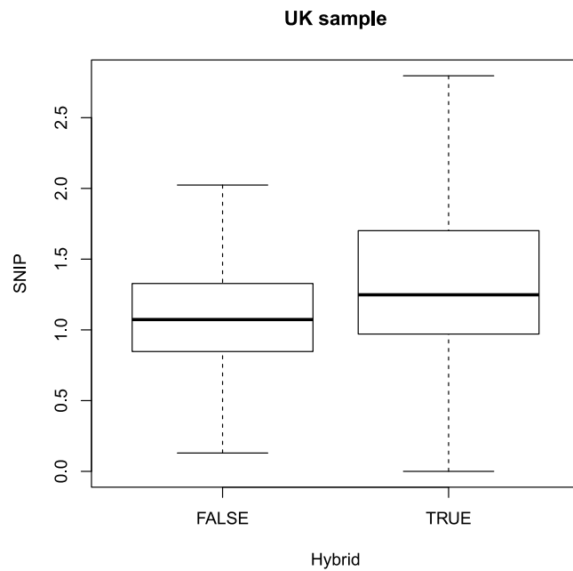
Figure 5. Box plots of SNIP for open-access and hybrid journals in 2017. Note: Outliers are not drawn.
