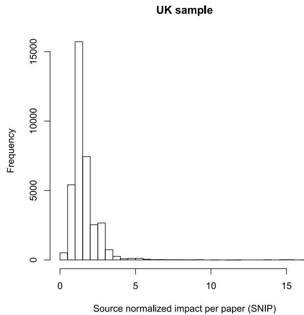
Figure 1. Histogram of SNIP for OpenAPC records.
