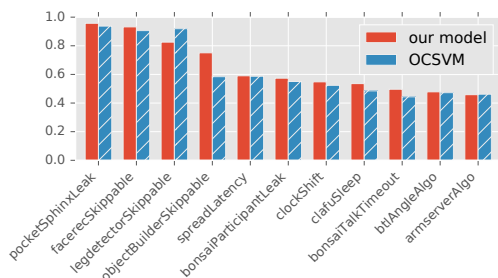
Fig. 4. The AUC scores for each fault kind contained in the evaluation data set. Results have been averaged in case a fault affected multiple components. For details about the individual faults please refer to Wienke et al. [19].
