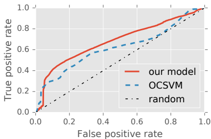
Fig. 3. ROC curves as micro-averages across components.
