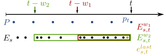
Fig. 2. Visualization of the feature generation and synchronization approach for a single scope s with two temporal windows w_1 (red) and w_2 (green). Features are computed for the performance counters (blue) p_t at time t . Rectangular regions indicate the events inside the respective window and the yellow event instance is the most recent one occurring before t .
