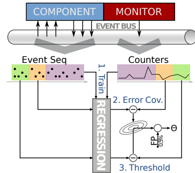
Fig. 1. Structural overview of the training of our approach. Colored region in the event and performance counter series indicate the different partitions of the training data used in sequential training steps.
