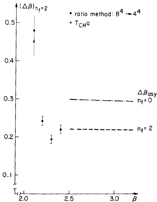
FIG. 2. \Delta\beta vs \beta for the SU(2) gauge theory with two flavors of dynamical fermions. Shown are the results obtained from the ratio method for tree-level improved ratios (circles) and results from the chiral phase transition (cross) (Ref. 15). The dash-dotted line shows the asymptotic scaling prediction in the absence of dynamical quarks, while the dashed line is the expectation for two flavors: \Delta\beta = 0.2107 + 0.0258/\beta . At \beta = 2.1 the error bar indicates only the spread of the three basic ratios measured.
