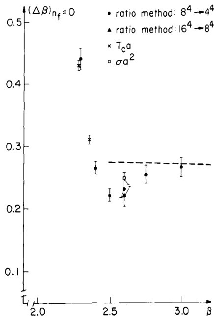
FIG. 1. Collection of the available information on \Delta\beta for the pure SU(2) gauge theory. Shown is \Delta\beta vs \beta obtained from the ratio method for tree-level improved ratios on a 8^4 lattice (circles) and 16^4 \rightarrow 8^4 lattice (triangle). Also shown are data taken from measurements of the deconfinement temperature (crosses) (from Refs. 10 and 11) and the string tension (square) (from Refs. 8 and 9). The dashed line indicates the expectation based on the asymptotic scaling relation, Eq. (4): \Delta\beta = 0.2575 + 0.0403/\beta .
